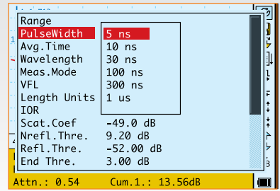
INSTRUMENT SETUP
