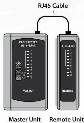
RJ45 Cable Connection
