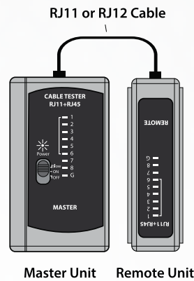
RJ11/RJ12 Cable Connection
